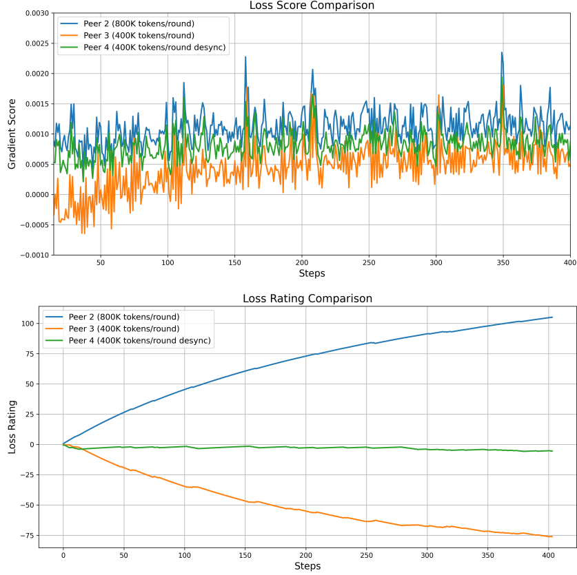
Figure 2: Simulating how the LossScore and LossRating evolves for three peers one processing more data and one desynchronized. We observe that variation in loss score is variable from step to step, however relative performance is consistent and the loss rating can quickly differentiate between peers with favorable behavior.
